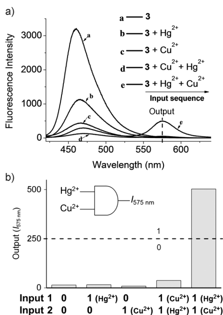
Figure 3. a) Fluorescence spectra of 3 (10 \mu\text{M} ) in \text{CH}_3\text{CN} under different input conditions; [ \text{Hg}^{2+} ] = 5 \mu\text{M} , [ \text{Cu}^{2+} ] = 10 \mu\text{M} ( \lambda_{\text{ex}} = 365 nm). b) Outputs in the fluorescence channel at 575 nm in response to two sequential inputs.
