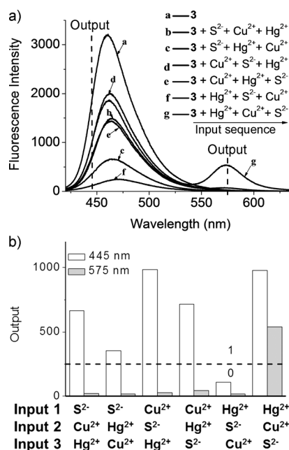
Figure 4. a) Fluorescence spectra of 3 (10 \mu\text{M} ) in \text{CH}_3\text{CN} under different input conditions; [ \text{Hg}^{2+} ] = 5 \mu\text{M} , [ \text{Cu}^{2+} ] = 10 \mu\text{M} , [ \text{S}^{2-} ] = 10 \mu\text{M} ( \lambda_{\text{ex}} = 365 nm). b) Outputs in the dual fluorescence channels at 445 and 575 nm in response to three sequential inputs.
